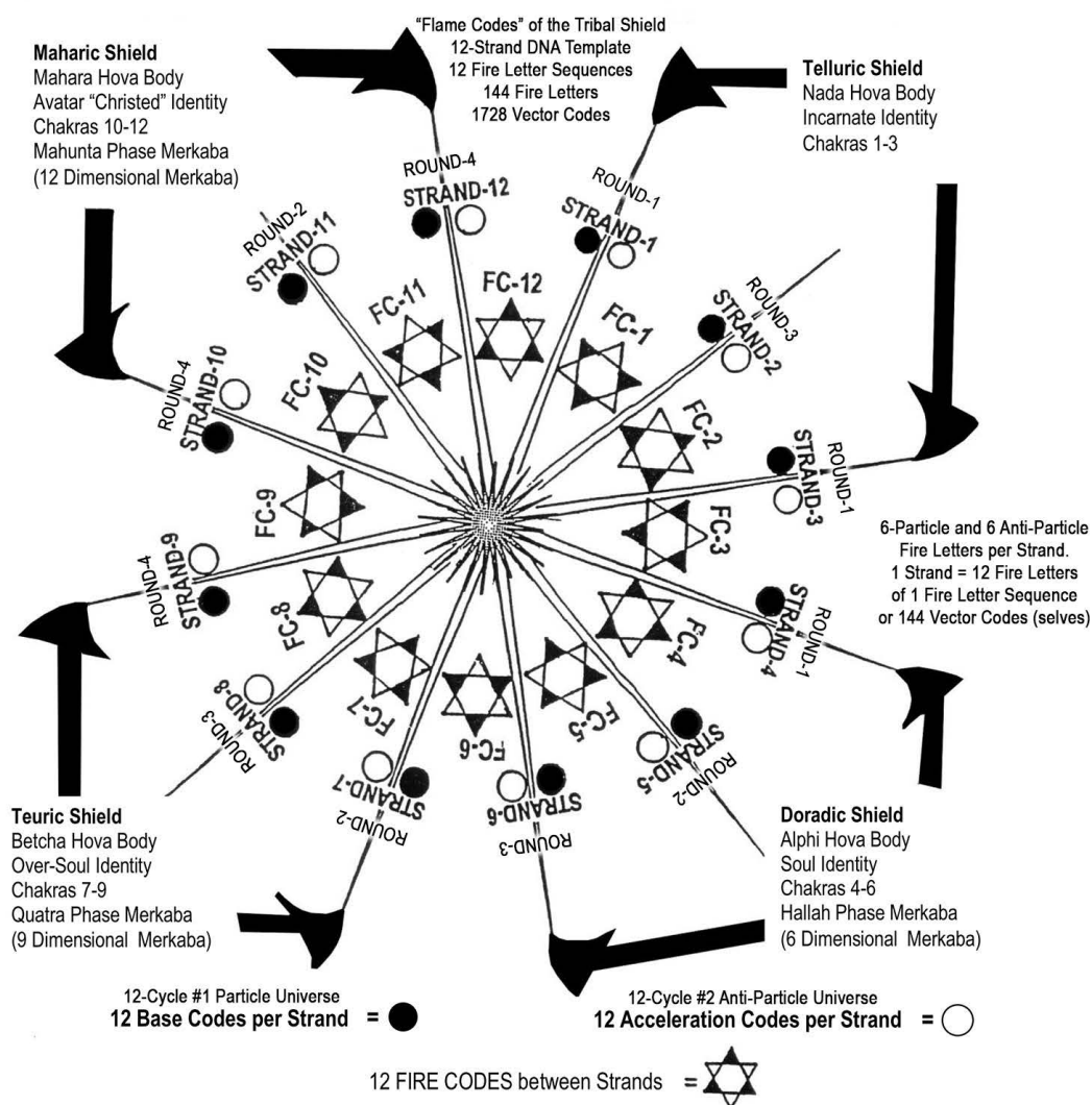
FIGURE 1. The Morphogenetic Field Scalar-Wave Template for the Original Human Genome
